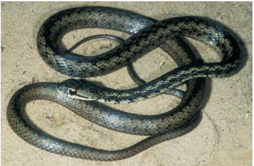
Fig. 2. Dorsolateral view of the holotype of Liopholidophis martae sp. n.
